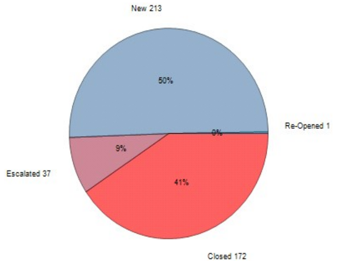
Violation Updates/Creates = 423
