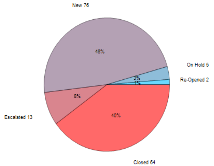
Violation Updates/Creates = 160
