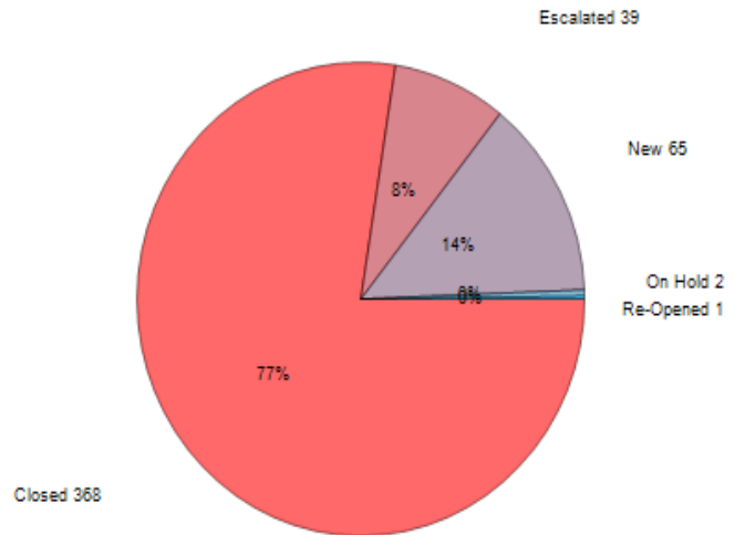
Violation Updates/Creates = 475
