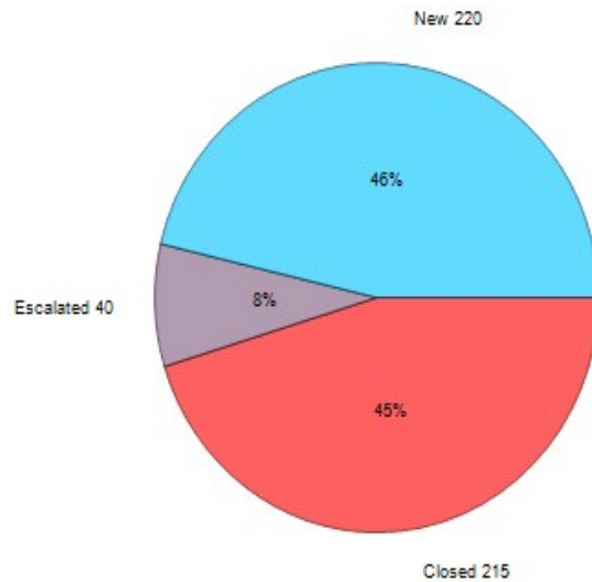
Violation Updates/Creates = 475
