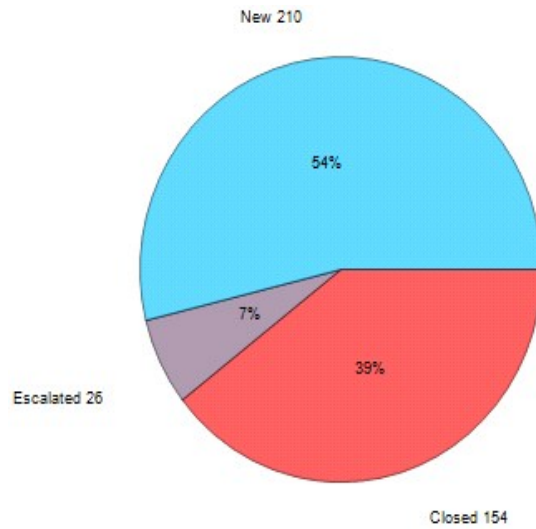
Violation Updates/Creates = 390
