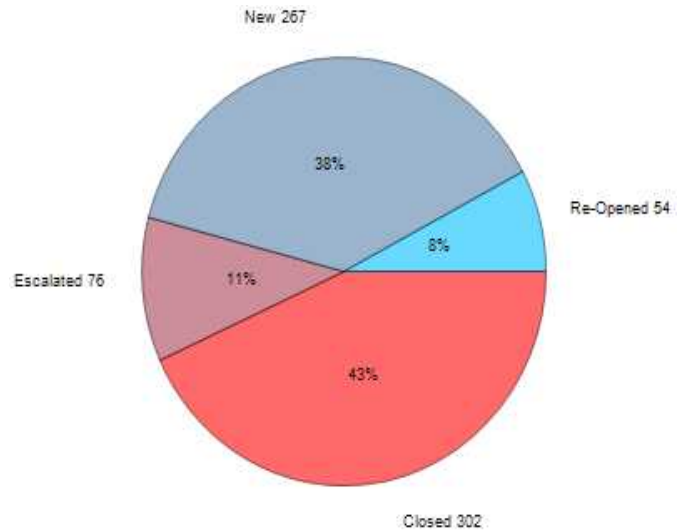
Violation Updates/Creates = 699
